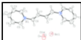
Fig. 1. The molecular structure of (I) showing the atom-labelling scheme. Displacement ellipsoids are drawn at the 50% probability level. Symmetry code of C7 a : -x + 1, -y, -z + 1 .
